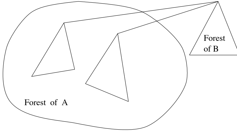
Figure 1: The forest of questions of A \rightarrow B .
