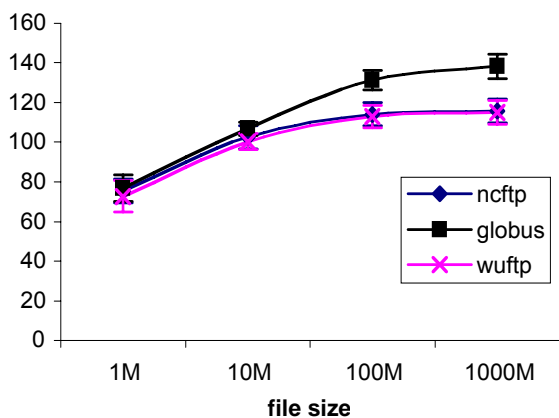
Figure 3: Single-stream throughput on LAN
