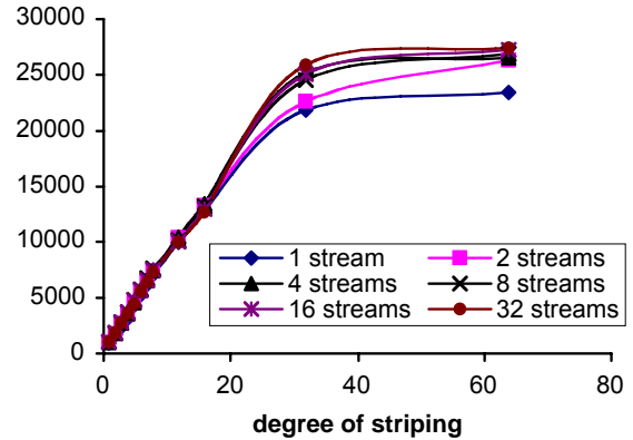
Figure 9: Globus mem-to-mem WAN performance
