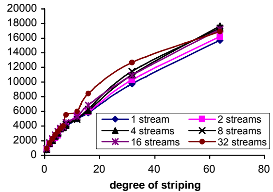
Figure 10: Globus disk-to-disk WAN performance
