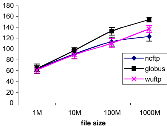
Figure 4: Single-stream throughput on WAN
