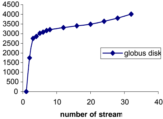
Figure 8: Seek operations at receiver vs. number of streams when transferring a 3 Gbyte file
