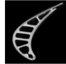
Figure 6.4: Cross-section of blade showing struts
