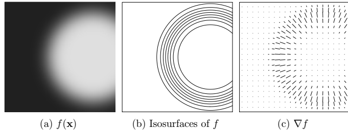
Figure 3.3: The gradient direction \nabla f (c) changes with position in the data (a), but it maintains its perpendicular orientation with respect to the isosurfaces (b).
