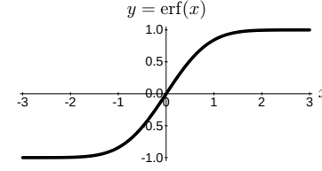
Figure 5.1: The error function, erf()
