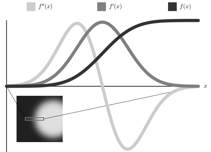
Figure 3.4: Ideal boundary analysis. The data value and its first and second derivatives are sampled along a short segment which passes through an object boundary
