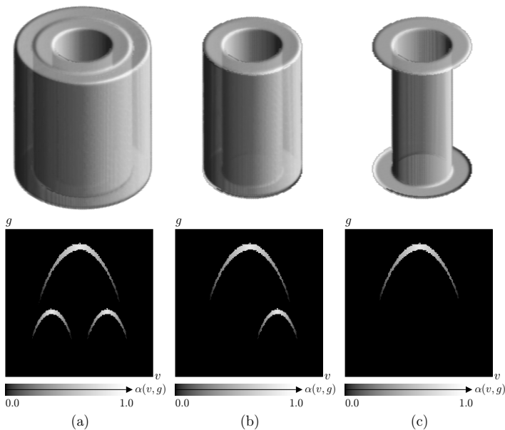
Figure 5.9: Renderings of nested cylinders and corresponding \alpha(v, g) . (a) shows the two dimensional opacity function \alpha(v, g) initially generated from Equation 5.13 and a simple b(x) . As with the scatterplots, the data value is on the horizontal axis, and gradient magnitude on the vertical. Black areas represent transparency; white is fully opaque. All three boundaries are visible in the corresponding rendering. By zeroing out areas in \alpha(v, g) , other boundaries can be removed with ease, as seen in (b) and (c).
