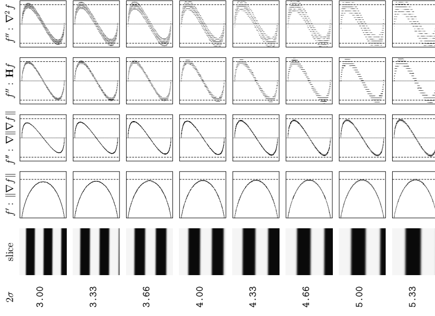
Figure C.4: Derivative measure comparisons for thicknesses 3.00 to 5.33
