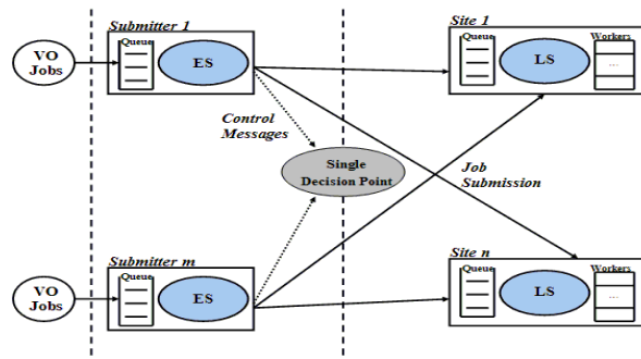
Figure 2: VO-Level Architecture
