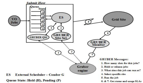
Figure 3: GRUBER Architecture
