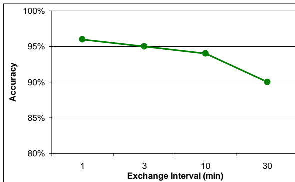
Figure 8: GT3 DI-GRUBER Scheduling Accuracy as Function of the Exchange Time Interval for Three Points
