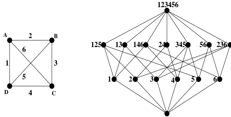
FIGURE 1. The graph K_4 and the lattice of flats of the corresponding matroid.
