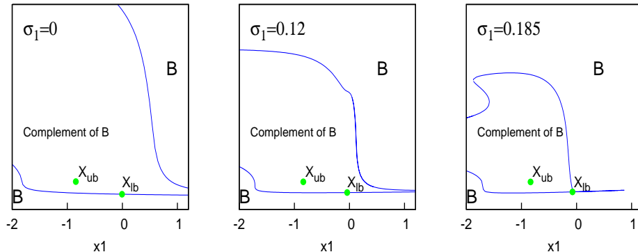
Figure 7: The ordinate is x_4 . For each value of \sigma_1 shown, there is a progressively narrower gap to the right of X_{lb} . Orbits starting above the narrower gap require longer to relaminarize than those starting below. It looks on this scale as if the gap closes when \sigma_1 = 0.185 , with X_{lb} falling on a critical point. A close up of the region near X_{lb} would show that this has not yet occurred for \sigma_1 = 0.185 , but see Figure 8.
