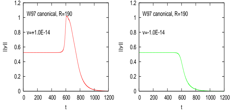
Figure 6: The model is W97 with the canonical values for the constants r_1 through \sigma_4 and R = 190 . The norms of orbits are shown on the interval [0, 1200] and v = \pm 10^{-14} . The two cases differ in the nature of the orbits and in the time for relaminarization to occur.
