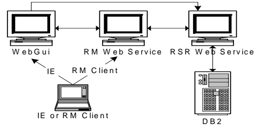
Figure 5. Deployment of the online matching system.
