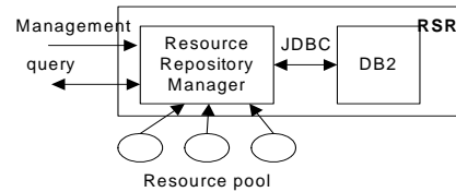
Figure 3. Structure of Resource State Repository
