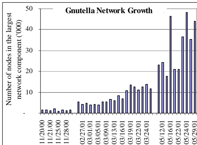
Figure 1: Gnutella network growth. The plot presents the number of nodes in the largest connected component in the network. Data collected during Nov. 2000, Feb./March 2001 and May 2001. We found a significantly larger network around Memorial Day (May 24-28) and Thanksgiving 2000, when apparently more people hunt for shared music online.
