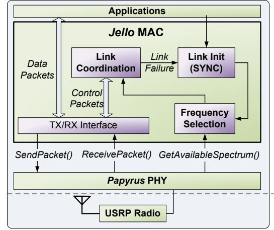
Figure 5: Jello and its interface with Papyrus.
