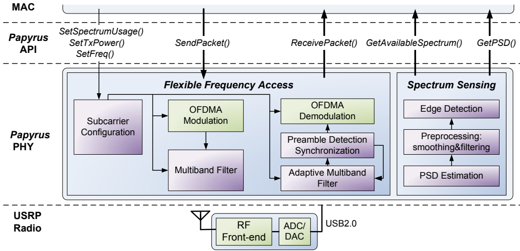
Figure 2: Papyrus software architecture and its interfaces with the MAC layer. Papyrus’s contributions are marked by the purple colored blocks.
