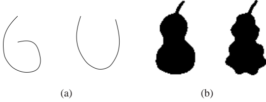
Figure 2. (a) Two curves that are almost indistinguishable by local properties alone. (b) Two objects that are similar at a coarse level but quite dissimilar at a local level.
