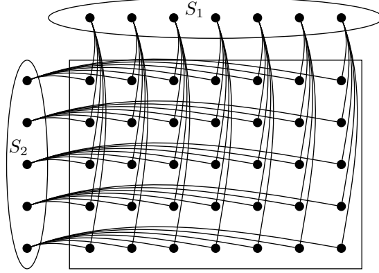
Figure 4: Constructing U(S_1, S_2) from the graphs S_1 and S_2 . The rectangle encloses the set of active vertices. (Edges within the S_i are not drawn.)
