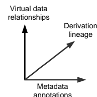
Figure 2: Query dimensions
