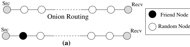
Fig. 1. Onion Routing path consists of randomly selected nodes. Our proposal, (a), has a friend node in the first position, with rest of the path members chosen randomly.
