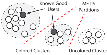
Figure 14: Unsupervised clustering with coloring.
