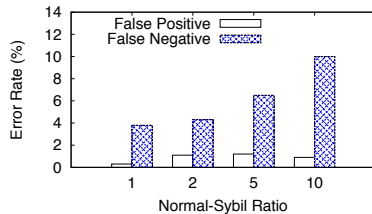
Figure 18: Detection accuracy versus Normal-Sybil ratio.
