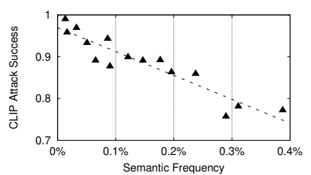
Figure 24. Success rate of the simple poisoning attack (rated by CLIP classifier) correlates strongly with concept sparsity measured by semantic frequency. Results for LD-CC. Same trend observed on SD-V2, SD-XL, DeepFloyd.
