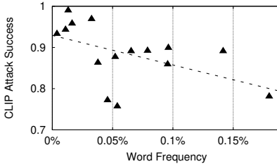
Figure 23. Success rate of the simple poisoning attack (rated by CLIP classifier) is weakly correlated with concept sparsity measured by word frequency in the training data. Results for LD-CC. Same trend observed on SD-V2, SD-XL, DeepFloyd.
